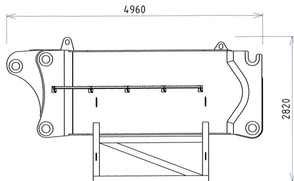
Boom extension adapter
