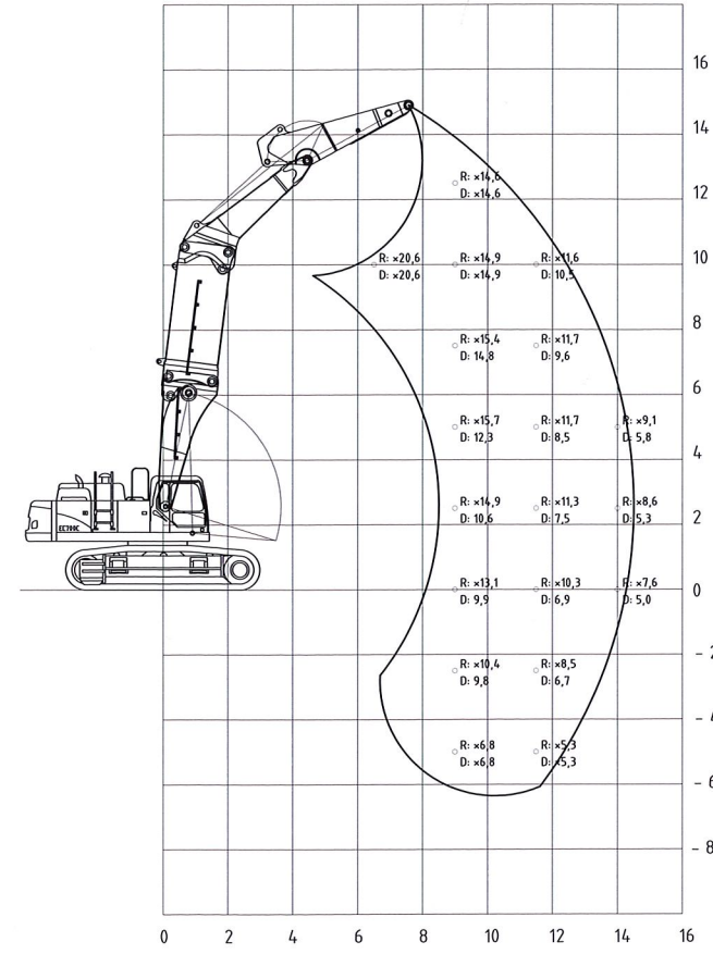
HRD front - Max. tool weight 2,5T
