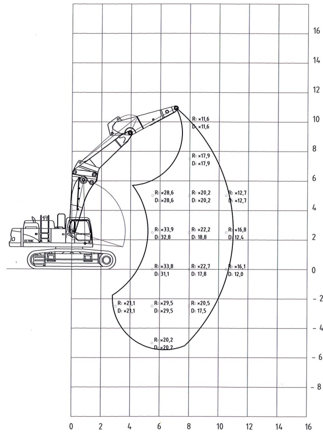
Digging front bent
