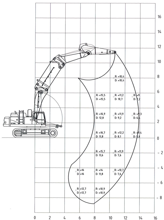
Digging front + boom extension/adapter - C
