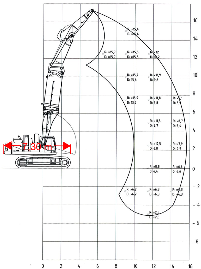
Digging front + boom extension/adapter - B
