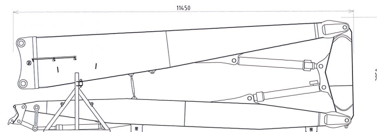
High Reach Demolition front
