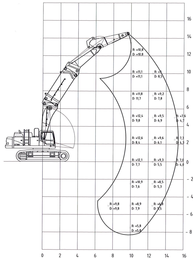
Digging front + boom extension/adapter - A
