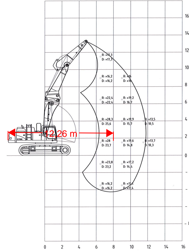
HRD front - Max. tool weight 3,5T
